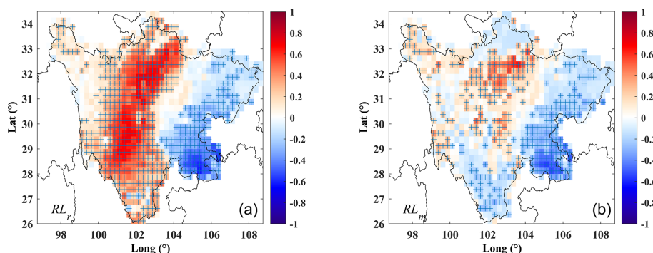
Figure 11. Same as in Fig. 3 but for RL_r (a) and RL_m (b).
