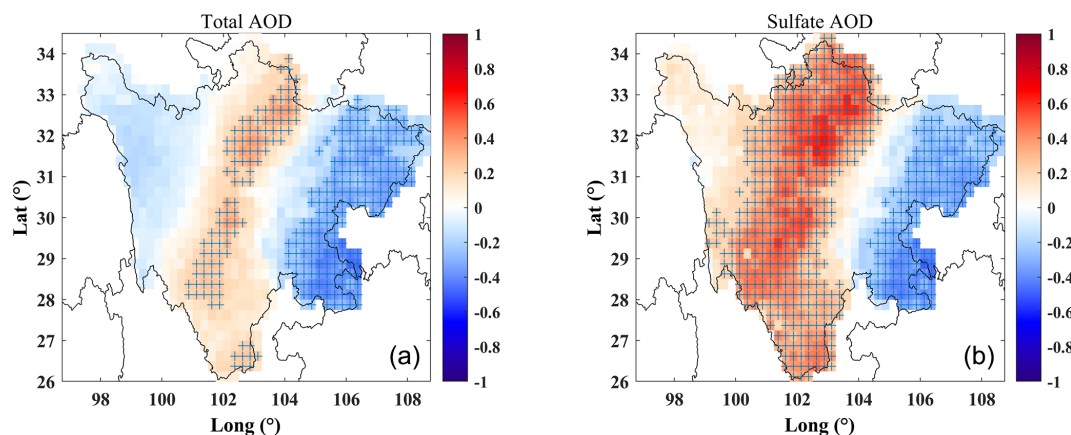
Figure 4. Pearson correlation coefficients between anomalies of total AOD and CG lightning (a) and anomalies of sulfate AOD and CG lightning (b) based on monthly data from 2005 to 2017. Crosses in the figure indicate grid boxes that have passed the 90 % significance test.
