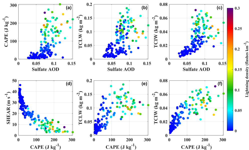
Figure 9. Joint effects of sulfate AOD and CAPE (a), sulfate AOD and TCLW (b), sulfate AOD and TCIW (c), CAPE and SHEAR (d), CAPE and TCLW (e), and CAPE and TCIW (f) on CG lightning density over the plateau region. The color of the dots represents the CG lightning density.
