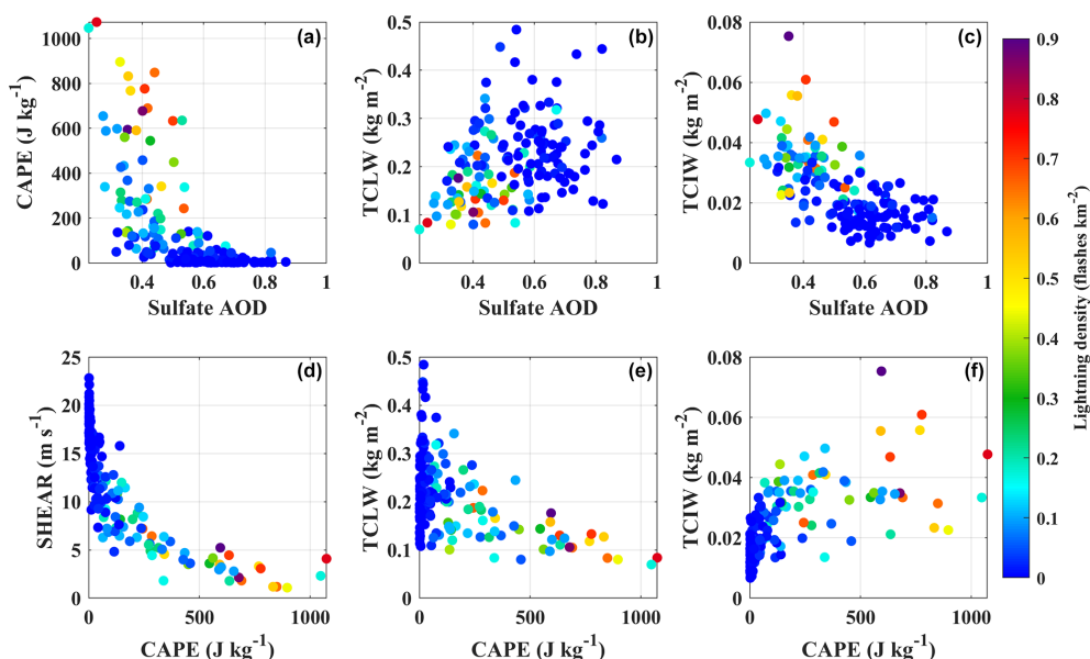
Figure 10. Same as in Fig. 9 but for the basin region.
