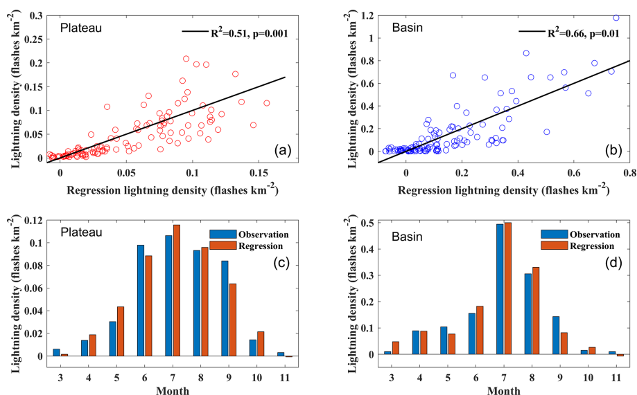
Figure 12. Scatterplots of observed CG lightning densities as a function of lightning densities from multiple linear regression in the plateau and basin regions (a, b) and their monthly distributions (c, d).
