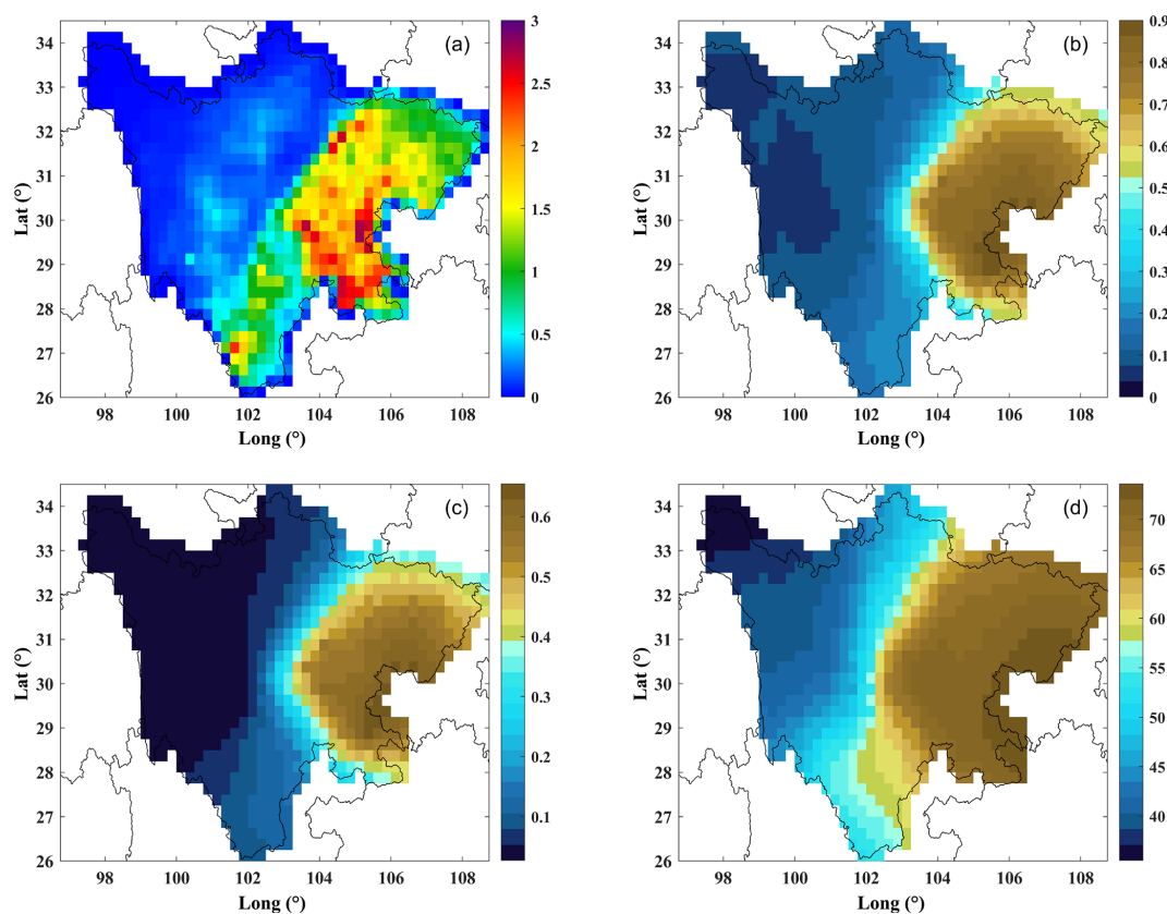
Figure 2. Distribution of (a) CG lightning density (unit: flashes \text{km}^{-2}\text{yr}^{-1} ), (b) total AOD, (c) sulfate AOD, and (d) the percentage of sulfate AOD in total AOD (unit: %) over Sichuan.
