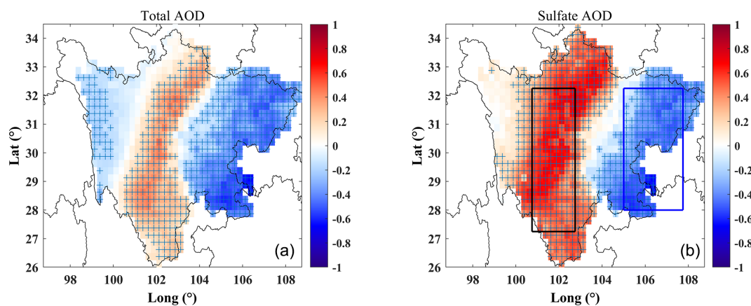
Figure 3. Pearson correlation coefficients between total AOD and CG lightning (a) and sulfate AOD and CG lightning (b) based on monthly data from 2005 to 2017. The correlation coefficient of each grid box is calculated from 156 monthly average data sets, and monthly average data are processed using a three-point moving average. Crosses in the figure indicate grid boxes that have passed the 95% significance test. The plateau region and the basin region are outlined by black and blue rectangles, respectively, in panel (b).
