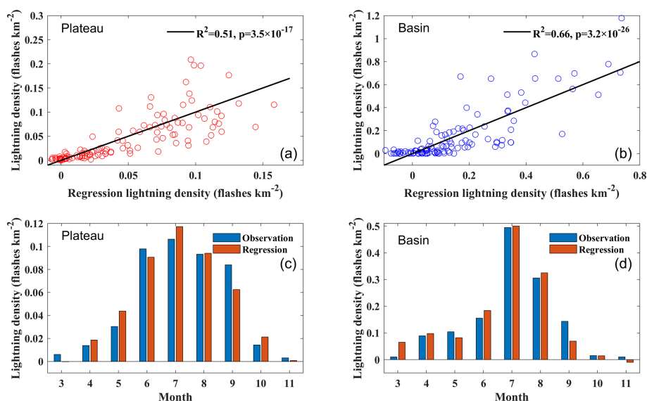
Figure 13. Scatterplots of observed CG lightning densities as a function of lightning densities from stepwise regression in the plateau and basin regions (a, b) and their monthly distributions (c, d).
