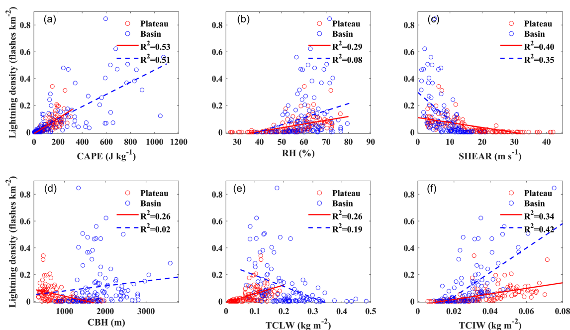
Figure 8. Lightning density as a function of thermodynamic and cloud-related factors in the basin (blue circles) and plateau (red circles) regions: (a) CAPE, (b) RH, (c) SHEAR, (d) CBH, (e) TCLW, and (f) TCIW. Linear-fit lines are shown, and coefficients of determination ( R^2 ) are given.
