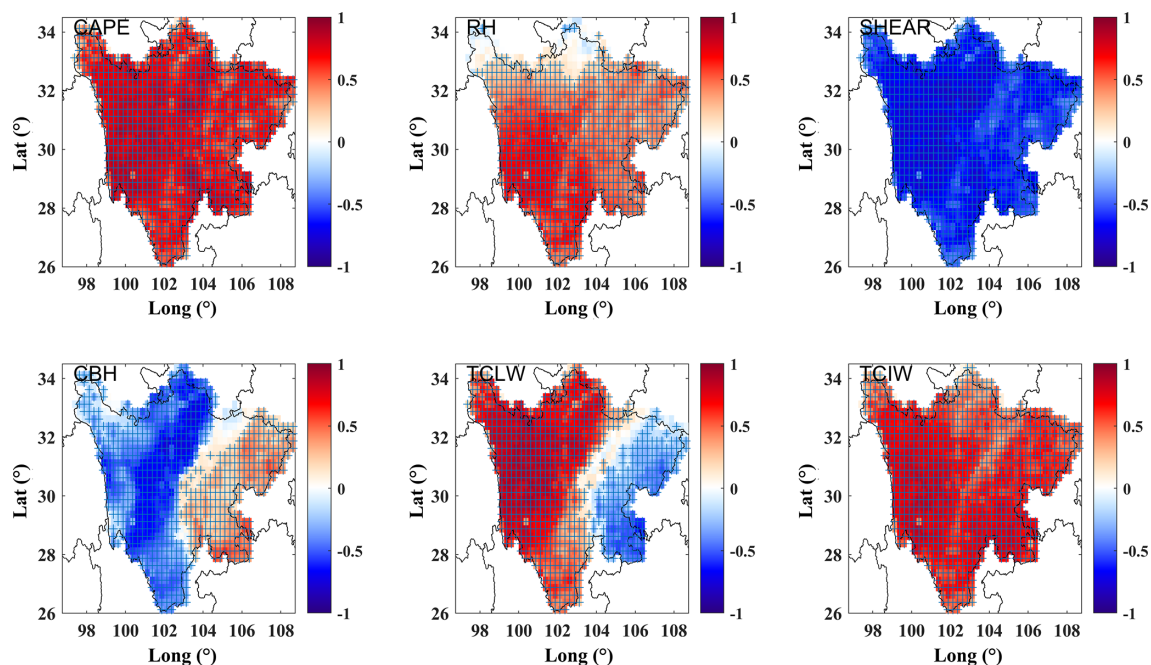
Figure 6. Pearson correlation coefficients of CAPE, RH, SHEAR, CBH, TCLW, and TCIW with CG lightning. Crosses in the figure indicate grid boxes that have passed the 95 % significance test.
