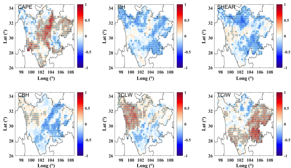
Figure 7. Partial correlation coefficients of CG lightning with thermodynamic and cloud-related factors, i.e., CAPE, RH, SHEAR, CBH, TCLW, and TCIW. Crosses in the figure indicate grid boxes that have passed the 95 % significance test.
