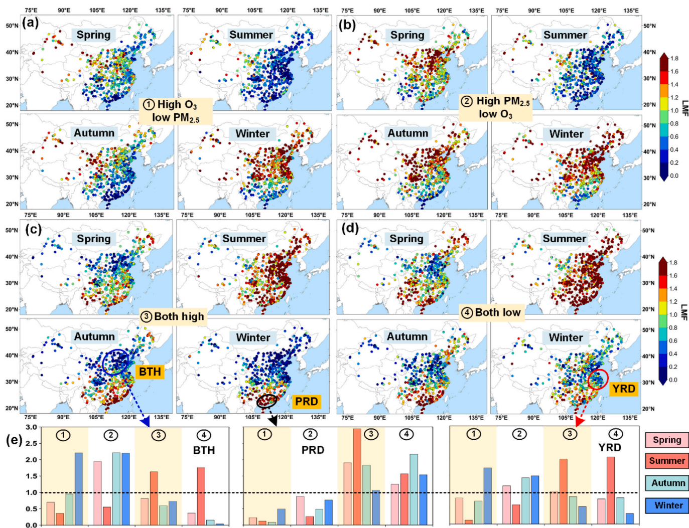
Fig. 3. (a)–(d) Mean LMF of four types of concurrent extreme O 3 and extreme PM 2.5 events in four seasons based on ground-based measurements during 2014–2021. The mean LMF in three mega-city regions: Beijing-Tianjin-Hebei (BTH; 37°–41°N, 114°–118°E), Yangtze River Delta (YRD; 30°–33°N, 118°–122°E) and Pearl River Delta (PRD; 21.5°–24°N, 112°–115.5°E). The black dotted line denotes where the LMF is 1.
