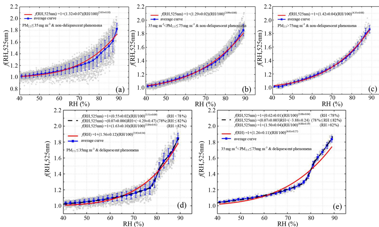
Figure 9. Fitted f(\text{RH}) of non-deliquestent curves (a–c) and deliquescent curves (d–e) for different pollution levels. Solid red lines represent fitted curves parameterized by Eq. (10). Dotted black lines represent the curves fit by segment function Eq. (12), and the solid blue lines represent the average curves.
