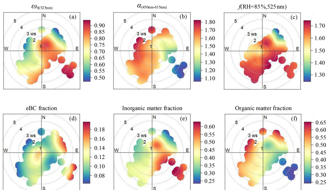
Figure 2. Wind dependence of (a) the single-scattering albedo ( \omega_0(525\text{ nm}) ), (b) the scattering Ångström exponent ( \alpha(450\text{--}635\text{ nm}) ), (c) the particle light scattering enhancement factor at RH = 85 % ( f(\text{RH} = 85\%, 525\text{ nm}) ), (d) the mass fraction of eBC, (e) the mass fraction of inorganic matter, and (f) the mass fraction of organic matter. The circular contours show the average change in wind speed and direction.
