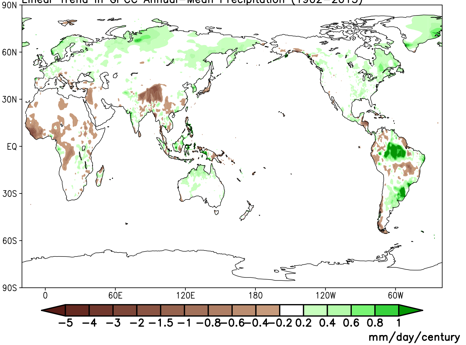
Linear Trend in GPCP Annual-Mean Precipitation (1902-2013)
