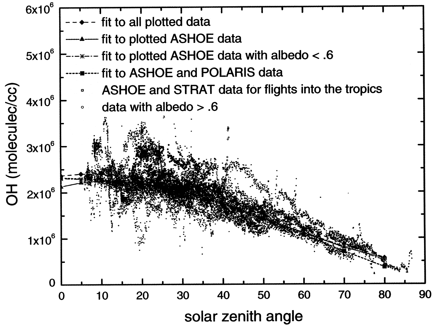
Plate 2. OH concentrations plotted as a function of solar zenith angle for data taken within 22° latitude of the equator for flights into the tropics during the ASHOE and STRAT campaigns. Data from those flights with albedo > 0.6 are plotted separately. Also shown are polynomial fits to all the data plotted, fits to subsets of the data as described in the legend, and a fit to all OH data from the ASHOE and POLARIS campaigns.
