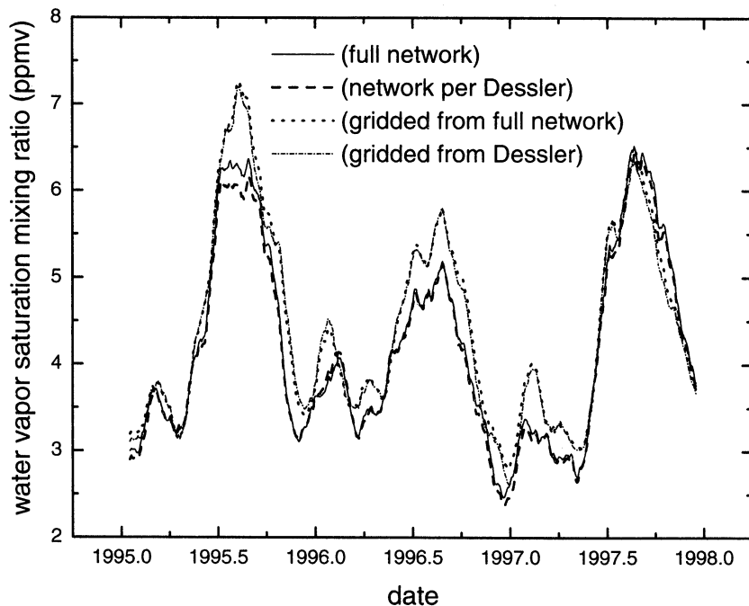
Figure 9. Plots of running mean WVSMRs derived from cold-point temperatures from radiosonde data between 10^{\circ}\text{S} and 10^{\circ}\text{N} . Shown are the average of all WVSMRs (solid line), the mean WVSMR of a grid onto which the individual minimum WVSMRs were interpolated (dotted line), a somewhat reduced number of stations, pruned to match the stations used by Dessler (dashed line), and the mean WVSMR of a grid onto which the individual minimum WVSMRs from the stations used by Dessler were interpolated (dotted-dashed line).
