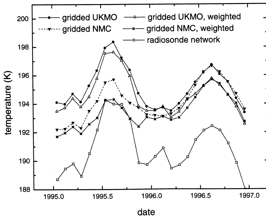
Figure 8. Monthly tropopause temperatures averaged from all radiosonde stations between 10^\circ\text{N} and 10^\circ\text{S} for 1995 and 1996. Plotted are monthly 100 mbar temperatures averaged using all NMC and UKMO grid points between 10^\circ\text{S} and 10^\circ\text{N} and monthly 100 mbar temperatures averaged using only NMC and UKMO grid points approximately collocated with tropical radiosonde stations.
