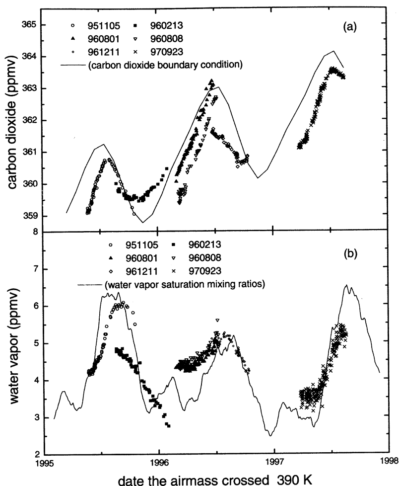
Figure 3. Mixing ratios measured above the tropopause plotted versus the date that the sampled air mass crossed the 390 K isentrope as determined by measured CO and the photochemical model: (a) carbon dioxide and (b) water vapor. Included in Figure 3a is a plot of (\text{CO}_2)_{bc} , boundary condition values determined from tropopause measurements as described in the text. Included in Figure 3b is a plot of running mean WWSMRs derived from cold-point temperatures from radiosonde data between 10^\circ\text{S} and 10^\circ\text{N} .
