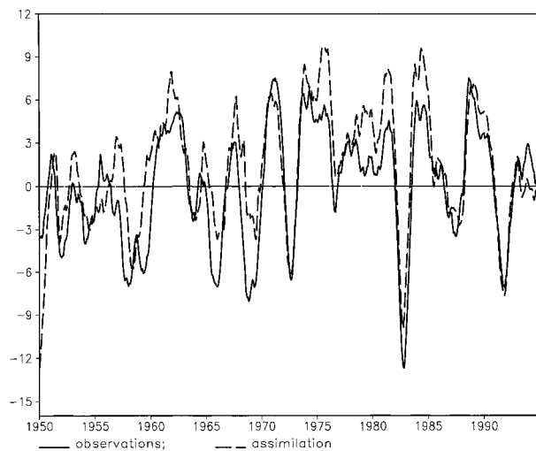
FIG. 1. Observed and control analysis sea level time series at Kwajalein Island ( 9^{\circ}\text{N} , 168^{\circ}\text{E} ). The seasonal cycle and a linear trend has been removed from both records.
