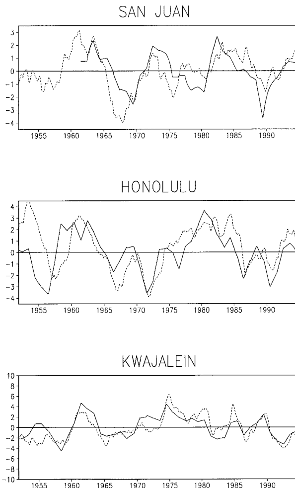
FIG. 2. Five-year low-pass filtered observed and control analysis sea level at three locations: San Juan, Puerto Rico ( 18^{\circ}\text{N} , 66^{\circ}\text{W} ), Honolulu ( 21^{\circ}\text{N} , 158^{\circ}\text{W} ), and Kwajalein Island ( 9^{\circ}\text{N} , 168^{\circ}\text{E} ). A linear trend has been removed from all records. Units are centimeters.
