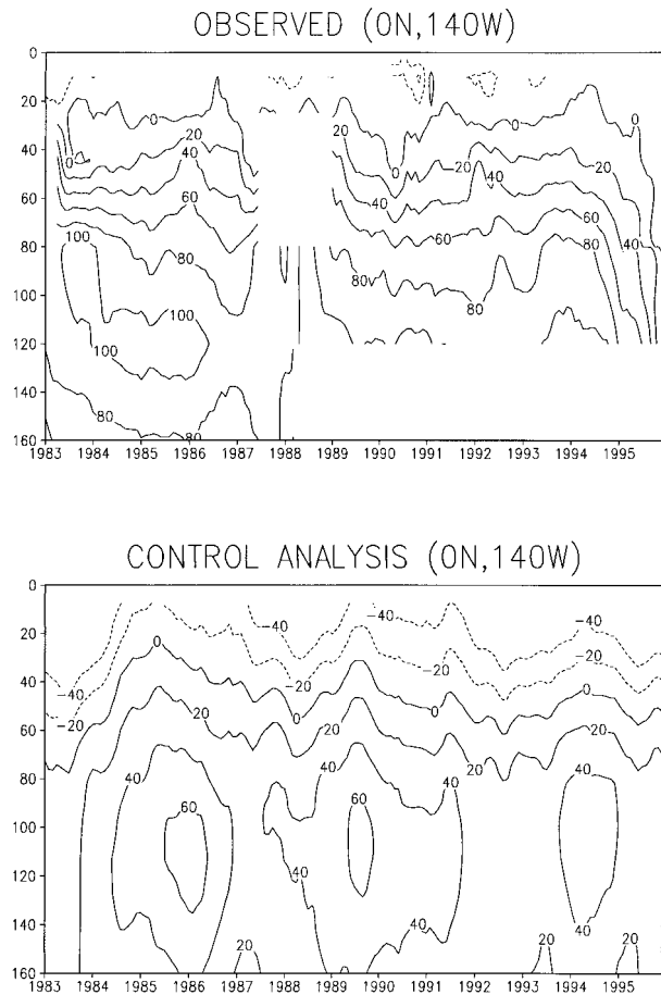
FIG. 6. Comparison of observed and control analysis zonal current time series on the equator with depth at 140°W in the eastern Pacific. Note the presence of strong interannual variability associated with El Niño.
