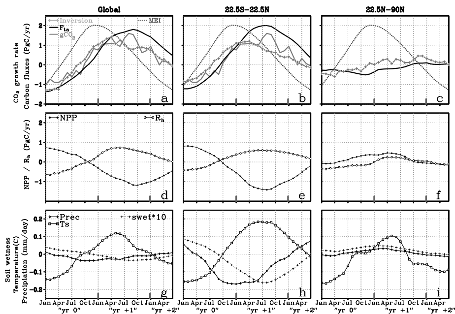
Fig. 4. Composites of the carbon fluxes and the climatic field anomalies during the growth, mature and decaying phases of ENSO. The left-hand (a, d, g), central (b, e, h) and right-hand (c, f, i) panels are the global, the tropical (22.5°S to 22.5°N) and Northern Hemispheric extratropics (22.5°N to 90°N) composites of the terrestrial fields, respectively. The top panels (a, b, c) are the terrestrial land–atmosphere carbon flux anomalies of VEGAS ( F_{ta} ) and inversion model, the atmospheric CO 2 growth rate ( gCO_2 ) and the reference MEI. The middle panels (d, e, f) are the corresponding Net Primary Production (NPP) and heterotrophic transpiration ( R_h ), and the bottom panels (g, h, i) are the observed temperature, precipitation and modelled soil wetness (Swet). Unit for carbon fluxes and CO 2 growth rate are PgCyr^{-1} , unit for precipitation is mm d^{-1} and temperature is °C, and MEI and soil wetness are non-dimensional. The notation of 'yr 0', 'yr +1', 'yr +2' is the same as in Rasmusson and Carpenter (1982) in which 'yr 0' is the mature phase of ENSO.
