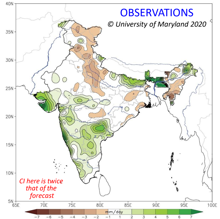
Figure 1. SST-based experimental forecast and verification of the 2020 Summer Monsoon (June-September) rainfall anomalies, with respect to the 1961-2010 climatology. The forecast is generated from regressions of the GPCP ver. 8 (Schneider et al. 2018) precipitation data on the SST principal components (Nigam et al. 2020) over the period 1901-2016. The forecast verification is generated from the IMD generated gridded rainfall (Pai et al. 2014). Green shading represents above-average rainfall while brown shading denotes below-average rainfall. The shading interval is 0.5 mm/day in the forecast and 1.0 mm/day in observations – all as indicated in the shading bar.
