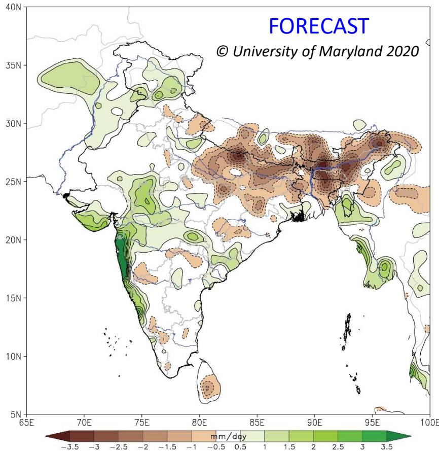
Figure 1. SST-based experimental forecast and verification of the 2020 Summer Monsoon (June-September) rainfall anomalies, with respect to the 1961-2010 climatology. The forecast is generated from regressions of the GPCP ver. 8 (Schneider et al. 2018) precipitation data on the SST principal components (Nigam et al. 2020) over the period 1901-2016. The forecast verification is generated from the IMD generated gridded rainfall (Pai et al. 2014). Green shading represents above-average rainfall while brown shading denotes below-average rainfall. The shading interval is 0.5 mm/day in the forecast and 1.0 mm/day in observations – all as indicated in the shading bar.
