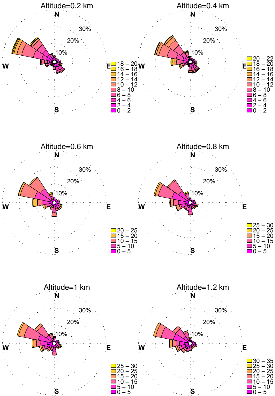
WINDROSES. PINEY RUN, MD WIND PROFILER. OCTOBER, HOURS: 12 pm to 15 pm DATA: FROM 1/2010 to 8/2014
