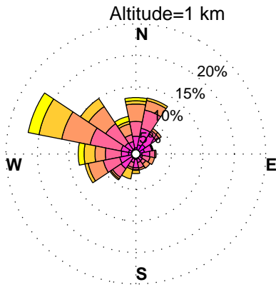
WINDROSES. PINEY RUN, MD WIND PROFILER. OCTOBER, HOURS: 12 am to 3 am DATA: FROM 1/2010 to 8/2014
