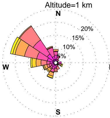
WINDROSES. PINEY RUN, MD WIND PROFILER. MARCH, HOURS: 12 am to 3 am DATA: FROM 1/2010 to 8/2014
