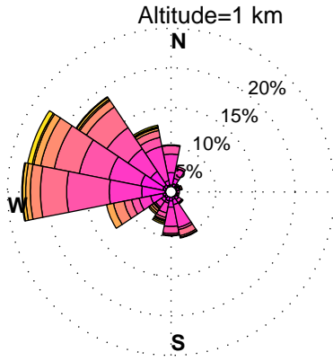
WINDROSES. PINEY RUN, MD WIND PROFILER. JULY, HOURS: 12 pm to 15 pm DATA: FROM 1/2010 to 8/2014
