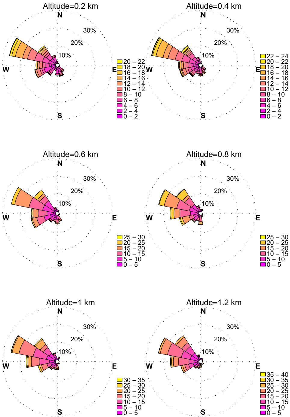
WINDROSES. PINEY RUN, MD WIND PROFILER. DECEMBER, HOURS: 12 pm to 15 pm DATA: FROM 1/2010 to 8/2014
