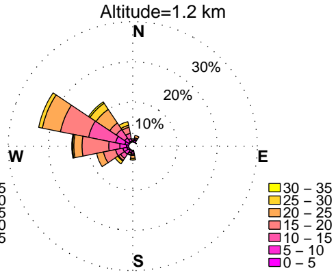
WINDROSES. PINEY RUN, MD WIND PROFILER. DECEMBER, HOURS: 12 am to 3 am DATA: FROM 1/2010 to 8/2014
