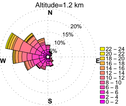
WINDROSES. PINEY RUN, MD WIND PROFILER. AUGUST, HOURS: 12 am to 3 am DATA: FROM 1/2010 to 8/2014
