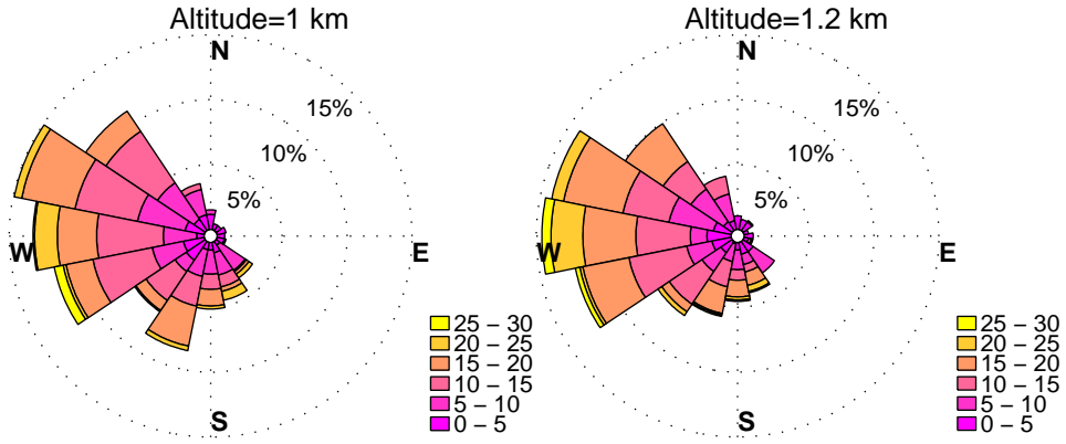
WINDROSES. PINEY RUN, MD WIND PROFILER. APRIL, HOURS: 12 pm to 15 pm DATA: FROM 1/2010 to 8/2014
