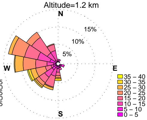
WINDROSES. PINEY RUN, MD WIND PROFILER. APRIL, HOURS: 12 am to 3 am DATA: FROM 1/2010 to 8/2014
