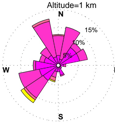
WINDROSES. HORN POINT, MD WIND PROFILER. SEPTEMBER, HOURS: 12 pm to 15 pm DATA: FROM 6/2012 to 6/2014
