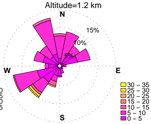
WINDROSES. HORN POINT, MD WIND PROFILER. SEPTEMBER, HOURS: 12 pm to 15 pm DATA: FROM 6/2012 to 6/2014
