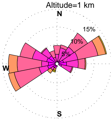
WINDROSES. HORN POINT, MD WIND PROFILER. SEPTEMBER, HOURS: 12 am to 3 am DATA: FROM 6/2012 to 6/2014
