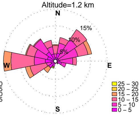
WINDROSES. HORN POINT, MD WIND PROFILER. SEPTEMBER, HOURS: 12 am to 3 am DATA: FROM 6/2012 to 6/2014
