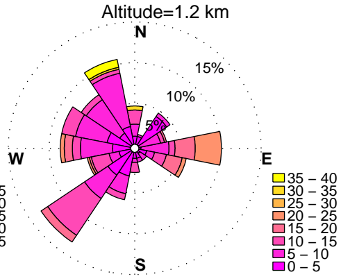
WINDROSES. HORN POINT, MD WIND PROFILER. OCTOBER, HOURS: 12 pm to 15 pm DATA: FROM 6/2012 to 6/2014
