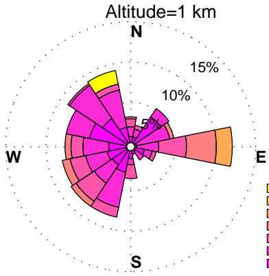
WINDROSES. HORN POINT, MD WIND PROFILER. OCTOBER, HOURS: 12 pm to 15 pm DATA: FROM 6/2012 to 6/2014
