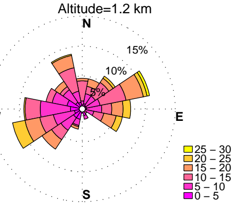
WINDROSES. HORN POINT, MD WIND PROFILER. OCTOBER, HOURS: 12 am to 3 am DATA: FROM 6/2012 to 6/2014
