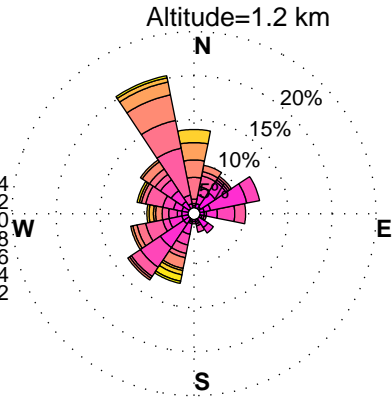
WINDROSES. HORN POINT, MD WIND PROFILER. NOVEMBER, HOURS: 12 pm to 15 pm DATA: FROM 6/2012 to 6/2014
