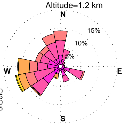
WINDROSES. HORN POINT, MD WIND PROFILER. MAY, HOURS: 12 am to 3 am DATA: FROM 6/2012 to 6/2014
