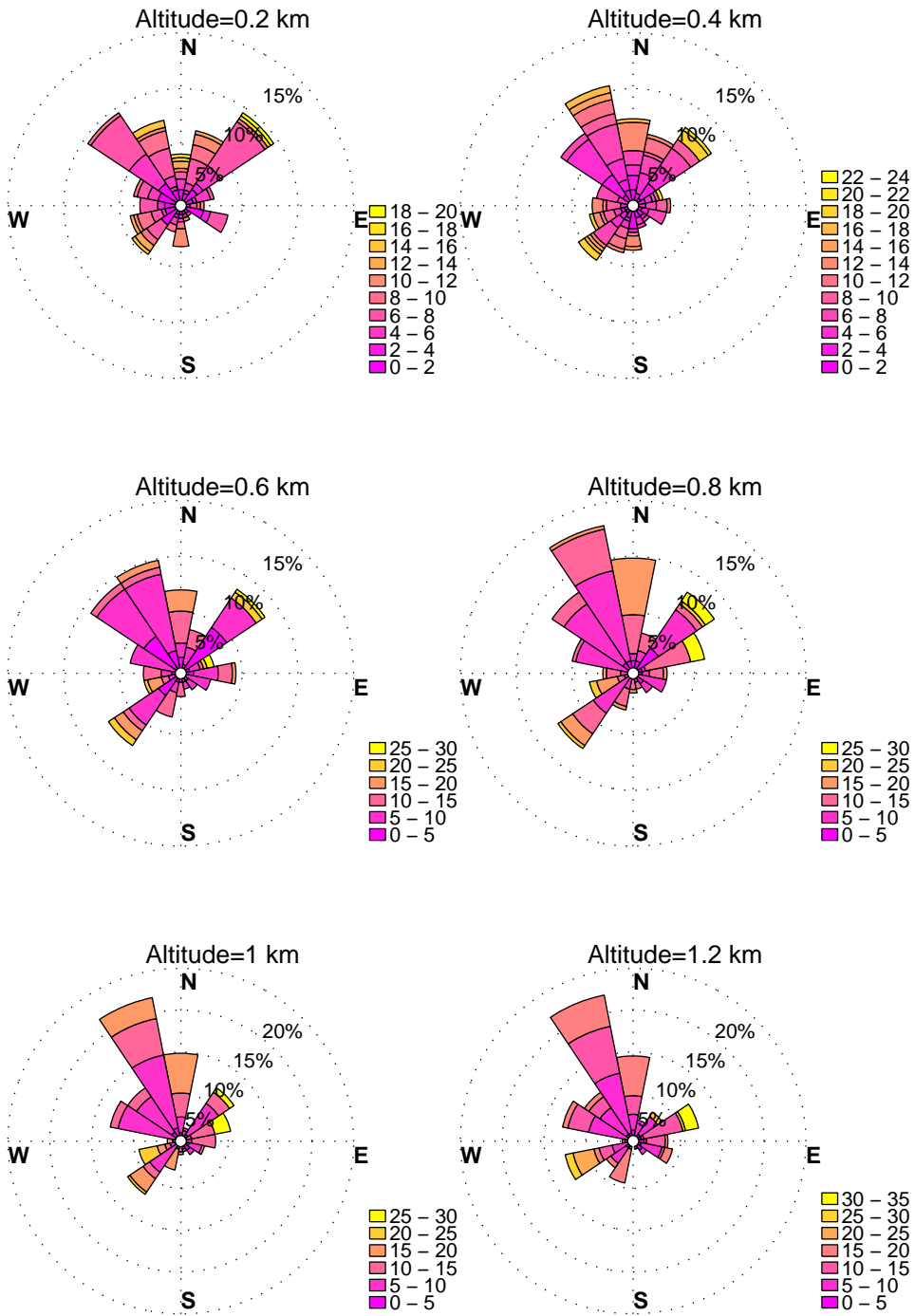
WINDROSES. HORN POINT, MD WIND PROFILER. MARCH, HOURS: 12 pm to 15 pm DATA: FROM 6/2012 to 6/2014
