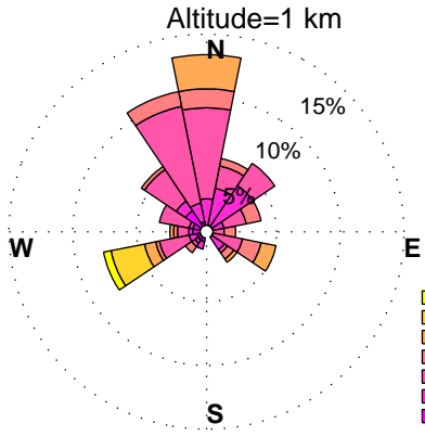
WINDROSES. HORN POINT, MD WIND PROFILER. MARCH, HOURS: 12 am to 3 am DATA: FROM 6/2012 to 6/2014
