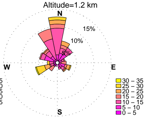
WINDROSES. HORN POINT, MD WIND PROFILER. MARCH, HOURS: 12 am to 3 am DATA: FROM 6/2012 to 6/2014
