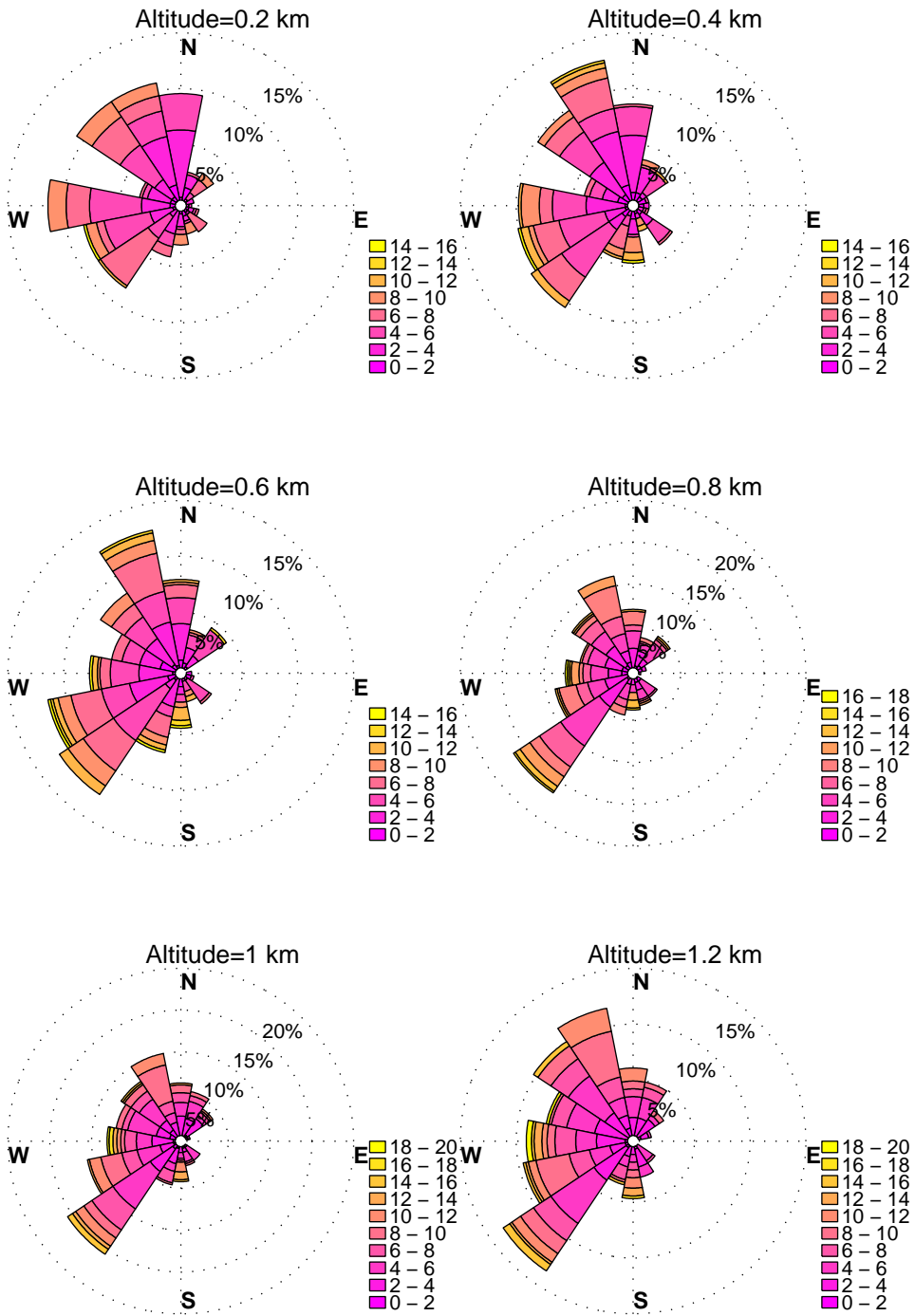
WINDROSES. HORN POINT, MD WIND PROFILER. JUNE, HOURS: 12 pm to 15 pm DATA: FROM 6/2012 to 6/2014
