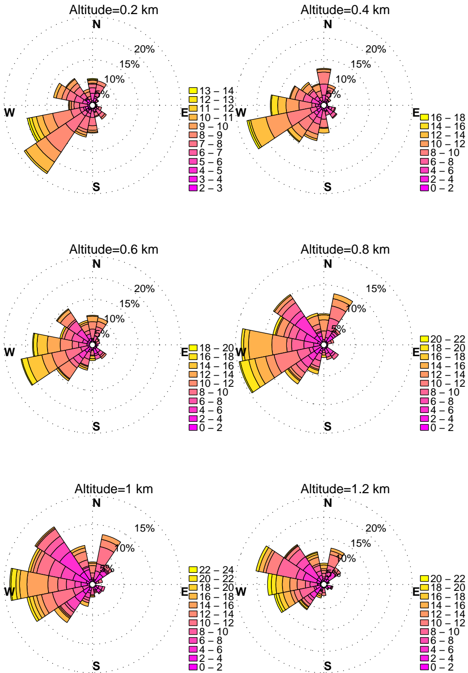
WINDROSES. HORN POINT, MD WIND PROFILER. JUNE, HOURS: 12 am to 3 am DATA: FROM 6/2012 to 6/2014
