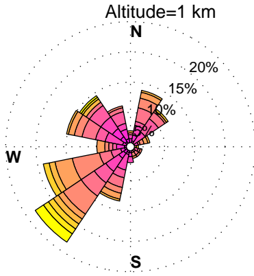
WINDROSES. HORN POINT, MD WIND PROFILER. JULY, HOURS: 12 pm to 15 pm DATA: FROM 6/2012 to 6/2014
