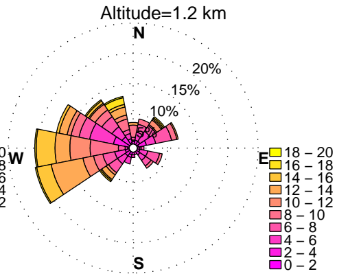
WINDROSES. HORN POINT, MD WIND PROFILER. JULY, HOURS: 12 am to 3 am DATA: FROM 6/2012 to 6/2014
