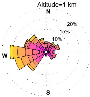
WINDROSES. HORN POINT, MD WIND PROFILER. JULY, HOURS: 12 am to 3 am DATA: FROM 6/2012 to 6/2014
