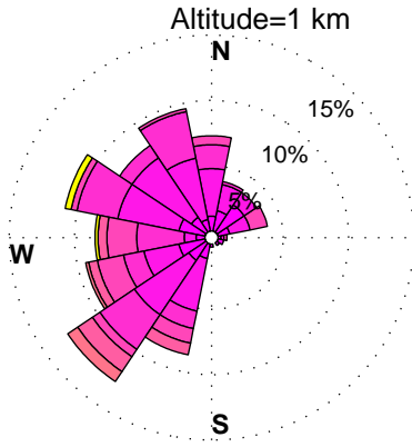
WINDROSES. HORN POINT, MD WIND PROFILER. JANUARY, HOURS: 12 pm to 15 pm DATA: FROM 6/2012 to 6/2014
