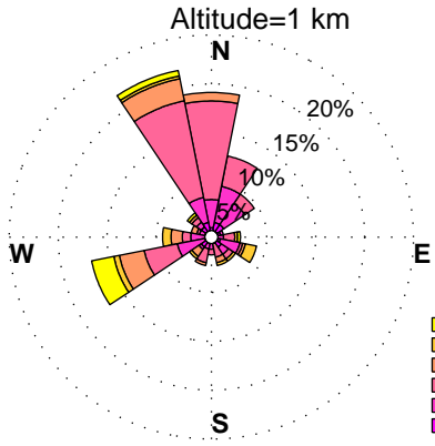
WINDROSES. HORN POINT, MD WIND PROFILER. FEBRUARY, HOURS: 12 am to 3 am DATA: FROM 6/2012 to 6/2014
