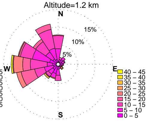
WINDROSES. HORN POINT, MD WIND PROFILER. DECEMBER, HOURS: 12 pm to 15 pm DATA: FROM 6/2012 to 6/2014
