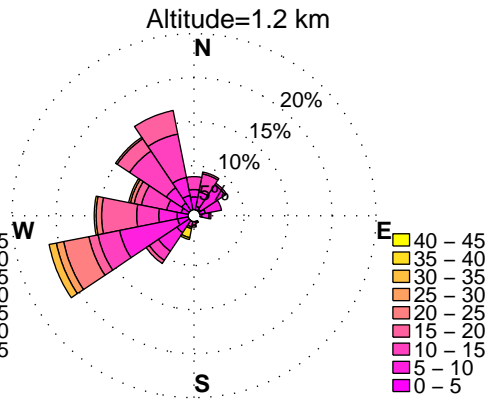
WINDROSES. HORN POINT, MD WIND PROFILER. DECEMBER, HOURS: 12 am to 3 am DATA: FROM 6/2012 to 6/2014
