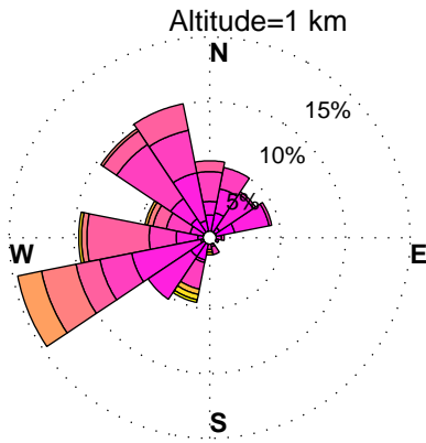
WINDROSES. HORN POINT, MD WIND PROFILER. DECEMBER, HOURS: 12 am to 3 am DATA: FROM 6/2012 to 6/2014
