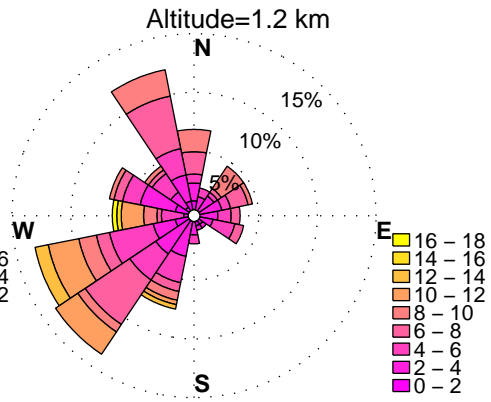
WINDROSES. HORN POINT, MD WIND PROFILER. AUGUST, HOURS: 12 pm to 15 pm DATA: FROM 6/2012 to 6/2014
