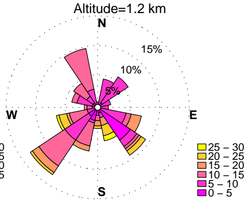
WINDROSES. HORN POINT, MD WIND PROFILER. APRIL, HOURS: 12 pm to 15 pm DATA: FROM 6/2012 to 6/2014
