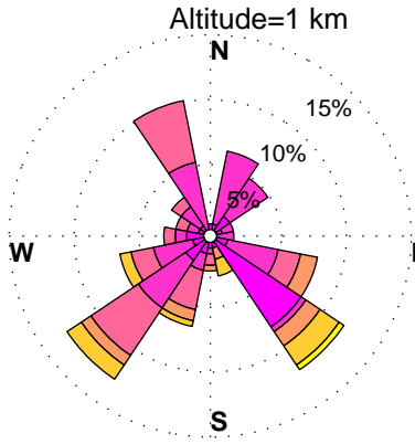
WINDROSES. HORN POINT, MD WIND PROFILER. APRIL, HOURS: 12 pm to 15 pm DATA: FROM 6/2012 to 6/2014
