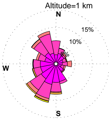
WINDROSES. BELTSVILLE, MD WIND PROFILER. SEPTEMBER, HOURS: 12 pm to 15 pm DATA: FROM 1/2010 to 9/2014
