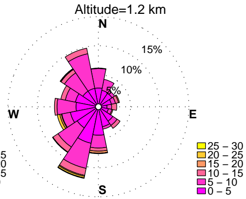
WINDROSES. BELTSVILLE, MD WIND PROFILER. SEPTEMBER, HOURS: 12 pm to 15 pm DATA: FROM 1/2010 to 9/2014
