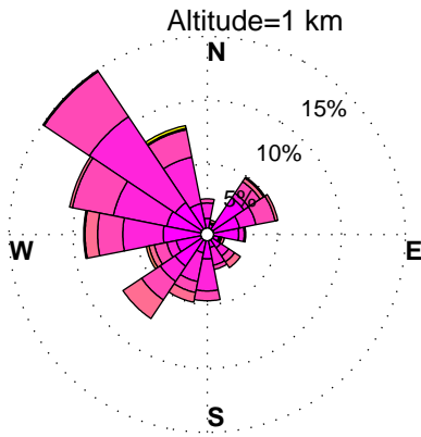
WINDROSES. BELTSVILLE, MD WIND PROFILER. OCTOBER, HOURS: 12 pm to 15 pm DATA: FROM 1/2010 to 9/2014
