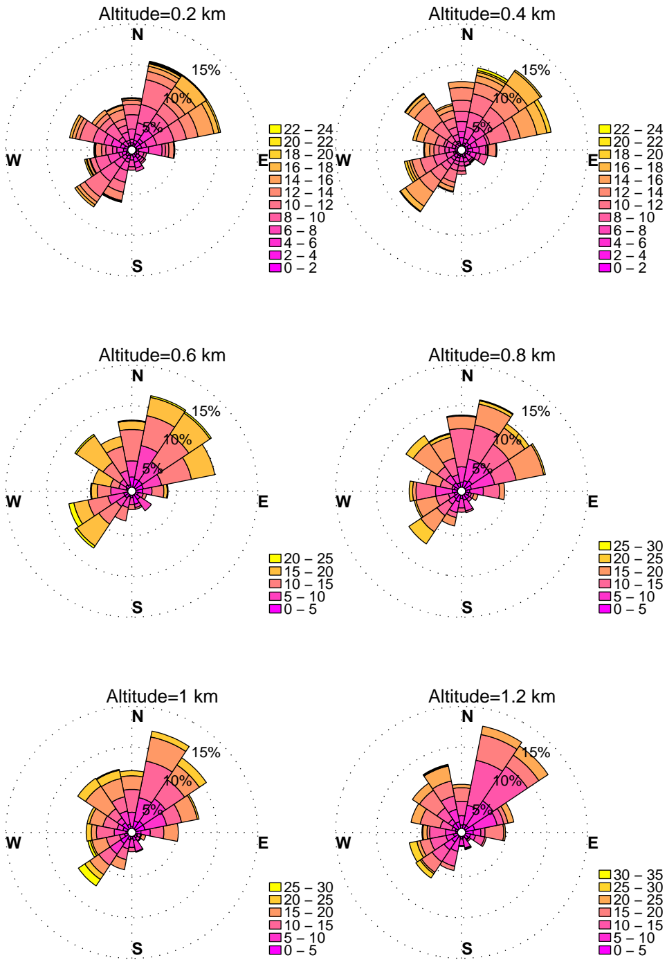
WINDROSES. BELTSVILLE, MD WIND PROFILER. OCTOBER, HOURS: 12 am to 3 am DATA: FROM 1/2010 to 9/2014
