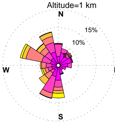
WINDROSES. BELTSVILLE, MD WIND PROFILER. NOVEMBER, HOURS: 12 pm to 15 pm DATA: FROM 1/2010 to 9/2014
