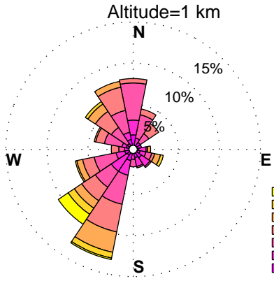
WINDROSES. BELTSVILLE, MD WIND PROFILER. MARCH, HOURS: 12 am to 3 am DATA: FROM 1/2010 to 9/2014
