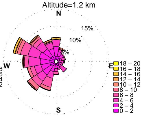
WINDROSES. BELTSVILLE, MD WIND PROFILER. JULY, HOURS: 12 pm to 15 pm DATA: FROM 1/2010 to 9/2014
