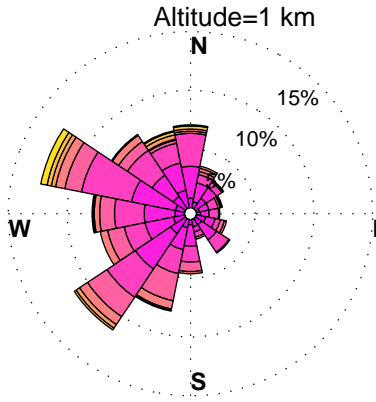
WINDROSES. BELTSVILLE, MD WIND PROFILER. JULY, HOURS: 12 pm to 15 pm DATA: FROM 1/2010 to 9/2014
