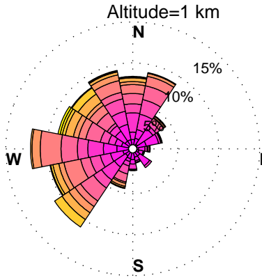
WINDROSES. BELTSVILLE, MD WIND PROFILER. JULY, HOURS: 12 am to 3 am DATA: FROM 1/2010 to 9/2014
