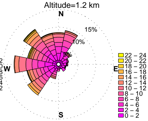
WINDROSES. BELTSVILLE, MD WIND PROFILER. JULY, HOURS: 12 am to 3 am DATA: FROM 1/2010 to 9/2014
