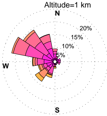
WINDROSES. BELTSVILLE, MD WIND PROFILER. JANUARY, HOURS: 12 am to 3 am DATA: FROM 1/2010 to 9/2014
