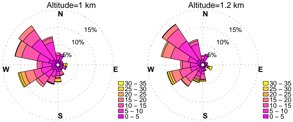
WINDROSES. BELTSVILLE, MD WIND PROFILER. DECEMBER, HOURS: 12 pm to 15 pm DATA: FROM 1/2010 to 9/2014
