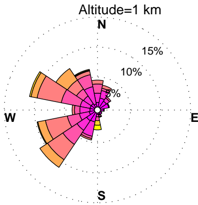
WINDROSES. BELTSVILLE, MD WIND PROFILER. DECEMBER, HOURS: 12 am to 3 am DATA: FROM 1/2010 to 9/2014
