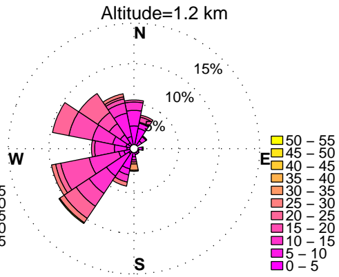
WINDROSES. BELTSVILLE, MD WIND PROFILER. DECEMBER, HOURS: 12 am to 3 am DATA: FROM 1/2010 to 9/2014
