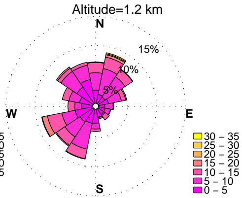
WINDROSES. BELTSVILLE, MD WIND PROFILER. AUGUST, HOURS: 12 am to 3 am DATA: FROM 1/2010 to 9/2014
