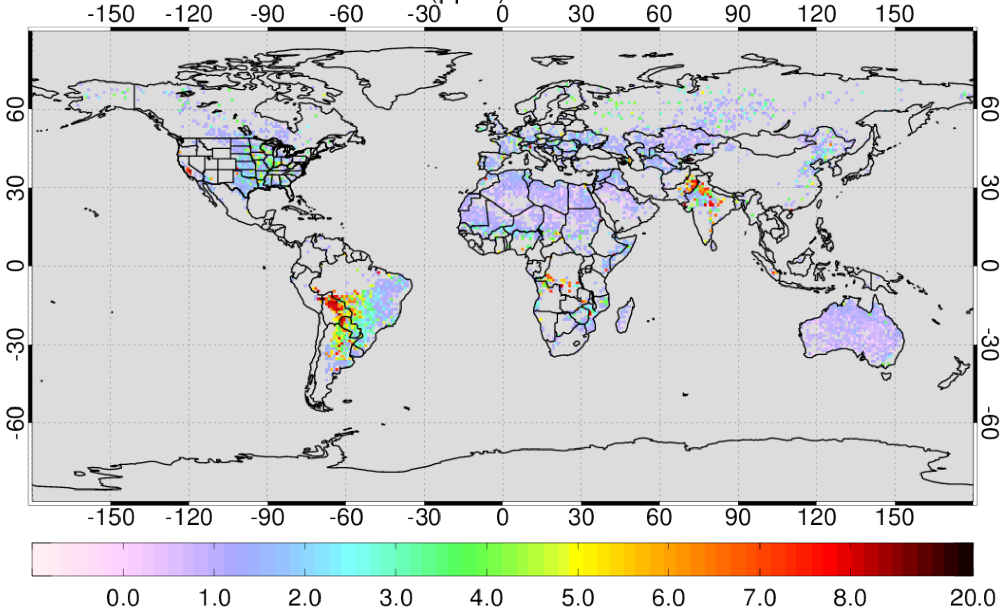
AIRS NH3 VMR (ppbv) at 918hPa for 201109
