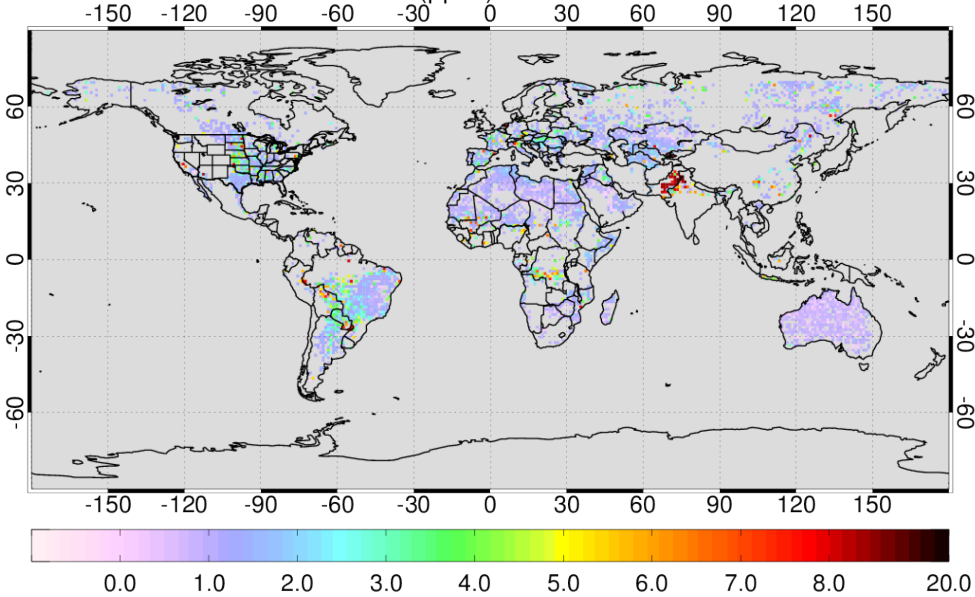
AIRS NH3 VMR (ppbv) at 918hPa for 201108
