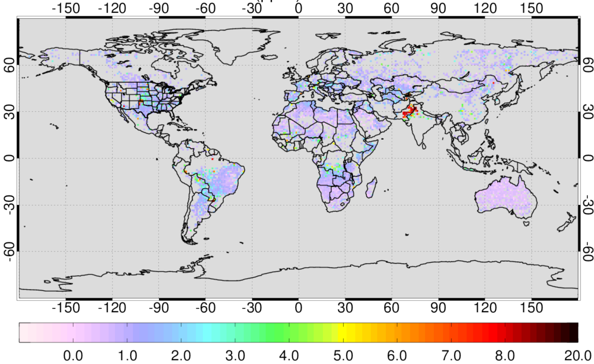
AIRS NH3 VMR (ppbv) at 840hPa for 201108
