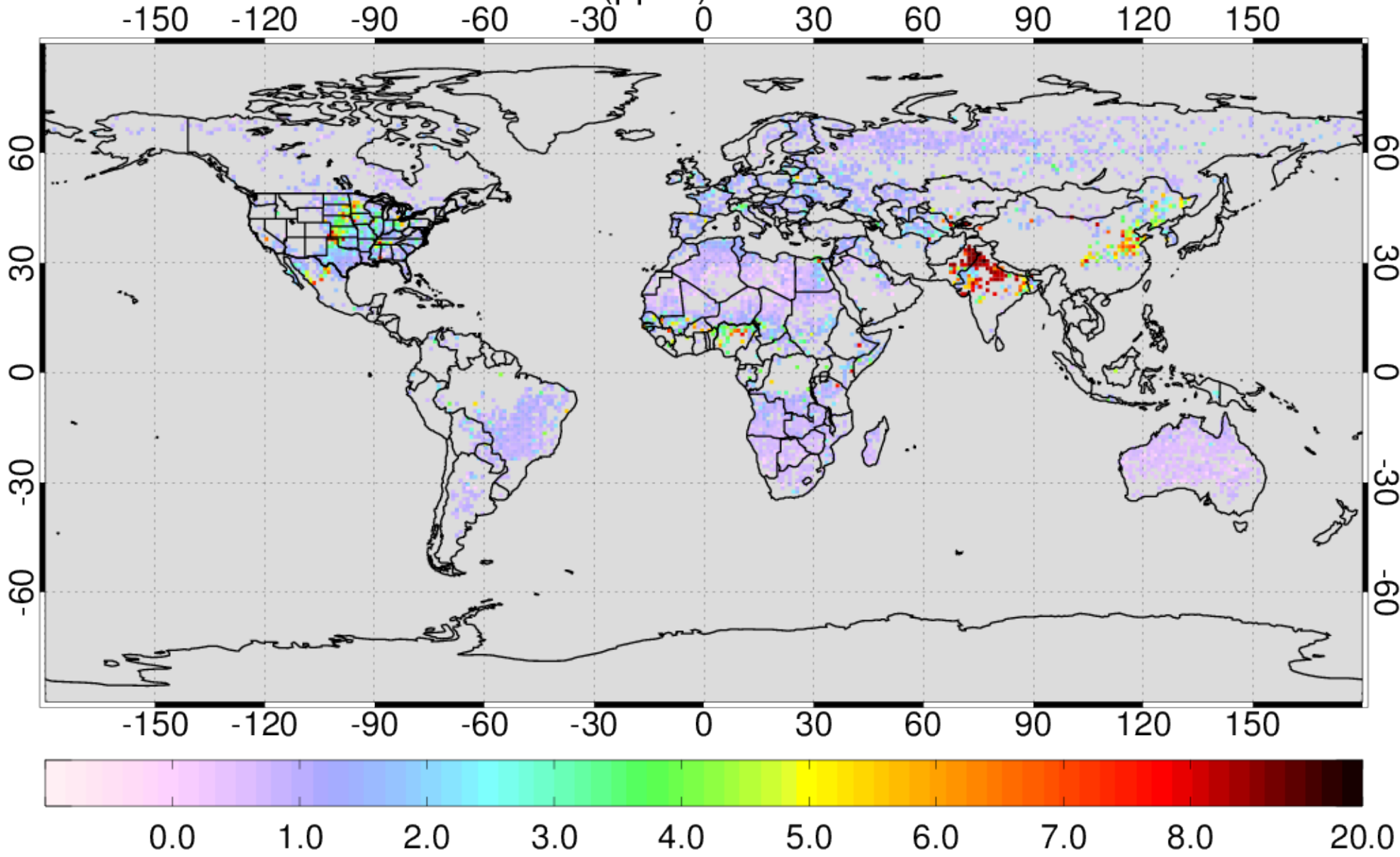
AIRS NH3 VMR (ppbv) at 840hPa for 201106
